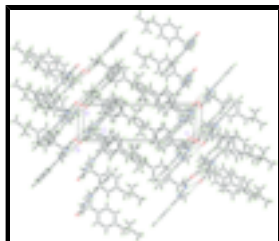
Fig. 2. The crystal packing of the title compound viewed down the b axis. Only the major disorder component is shown.
