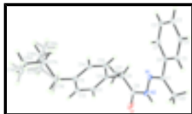
Fig. 1. The molecular structure of the title compound, showing 50% probability displacement ellipsoids and the atom-numbering scheme. Both disorder components are shown.
